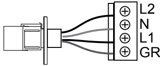
NORTH AMERICAN Figure 6.0c 240V 60Hz Wiring
